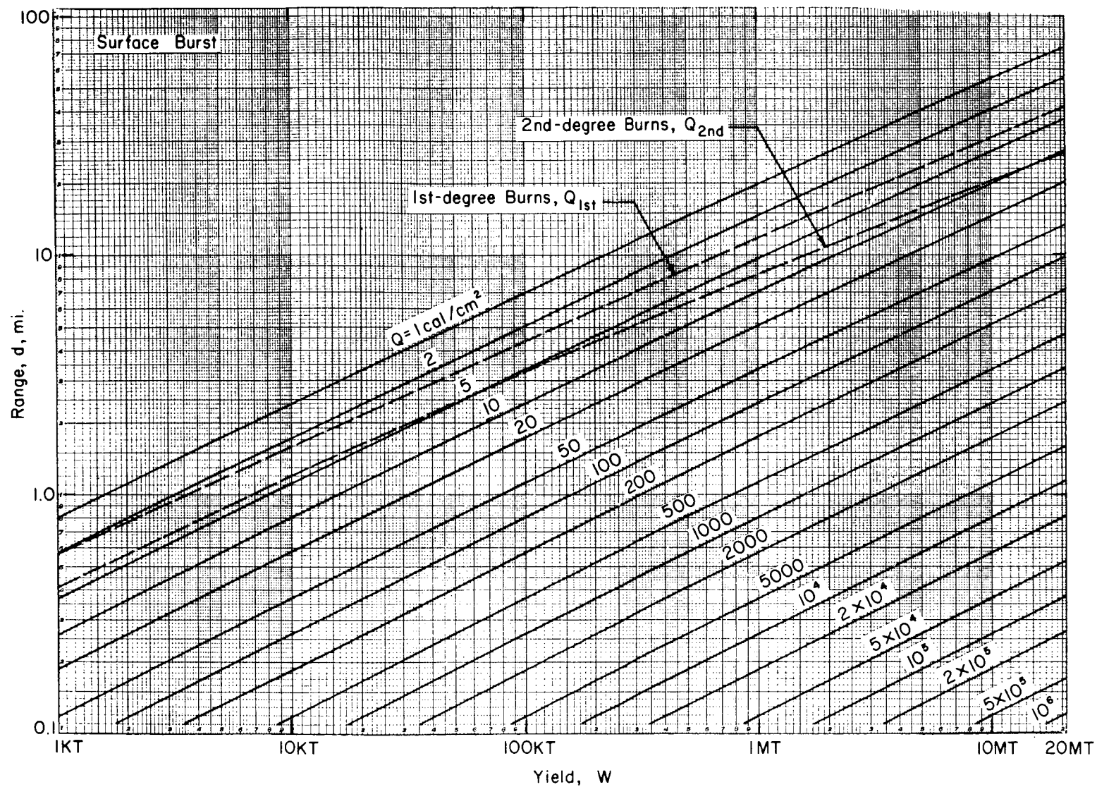
Fig. 2.13—Thermal radiation for surface bursts as a function of range and yield (50-mile visibility) and first- and second-degree burns for bare white skin vs. yield (see Eqs. 2.109 through 2.111 in Table 2.11).
